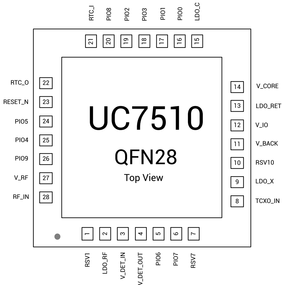
Figure 6-1 QFN28 Pin Assignment
