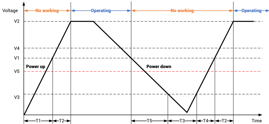
Figure 5-2 Power-up and Power-down Requirements
