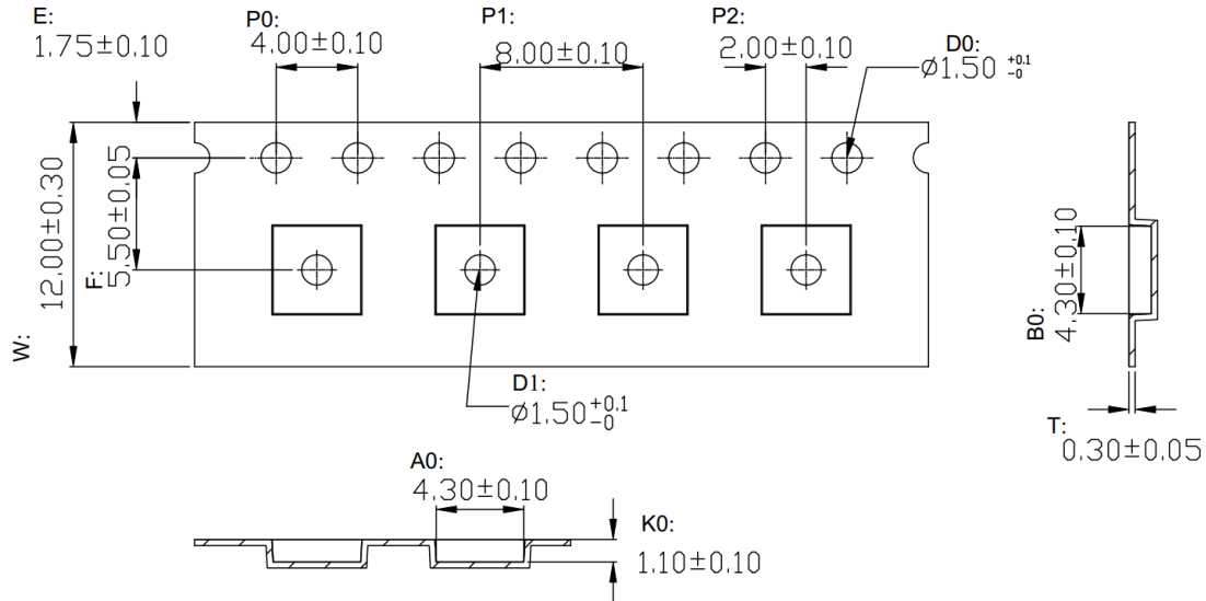
Figure 11-3 UC7510 Tape Dimensions (mm)
