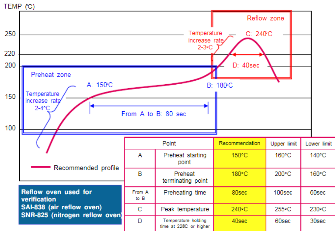
Figure 10-1 Reflow Soldering Temperature Curve
