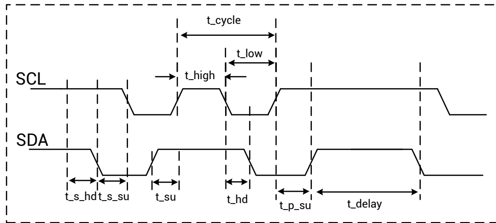
Figure 3-1 I2C Timing Requirements
