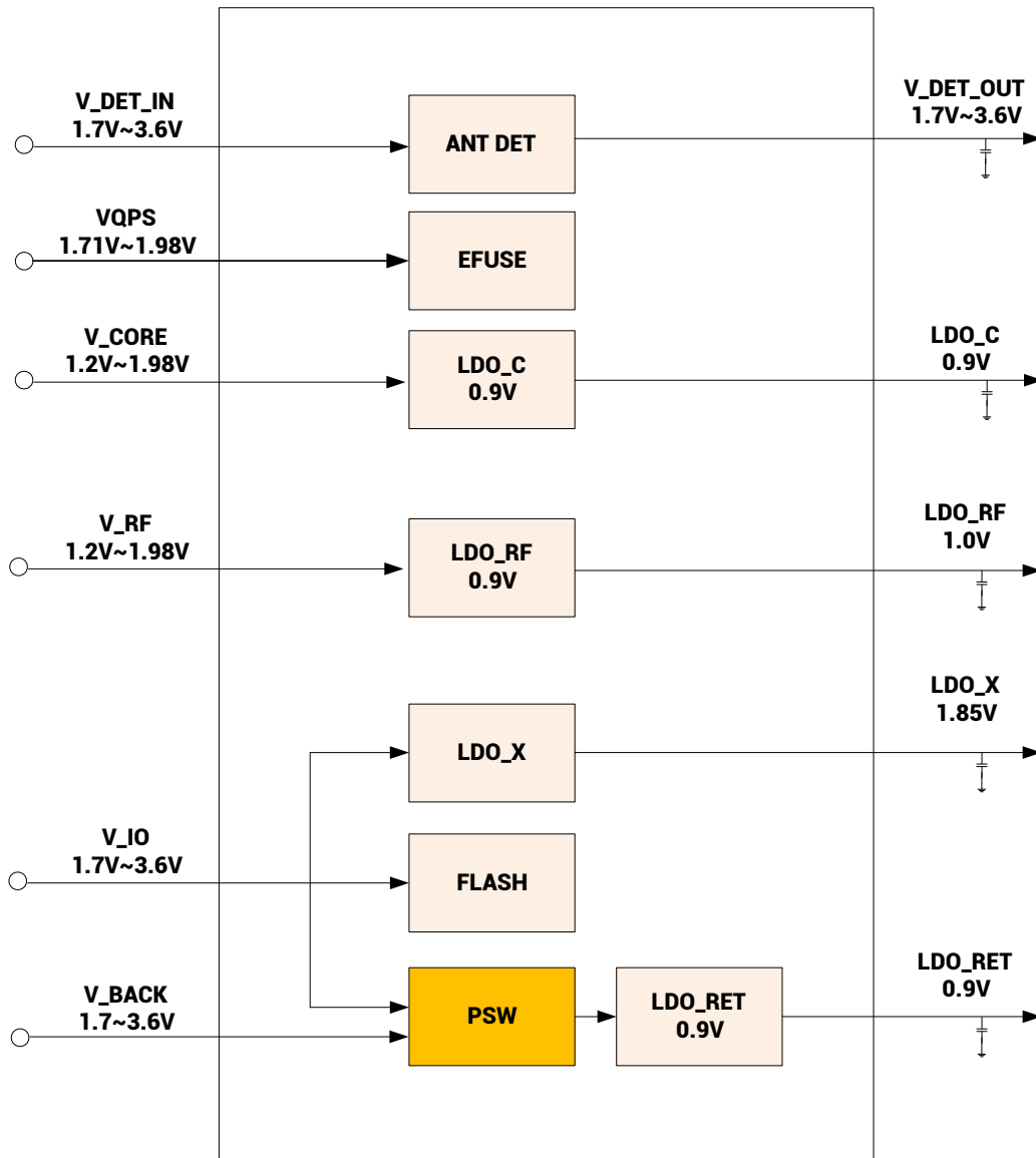
Figure 5-1 Power Management Unit
