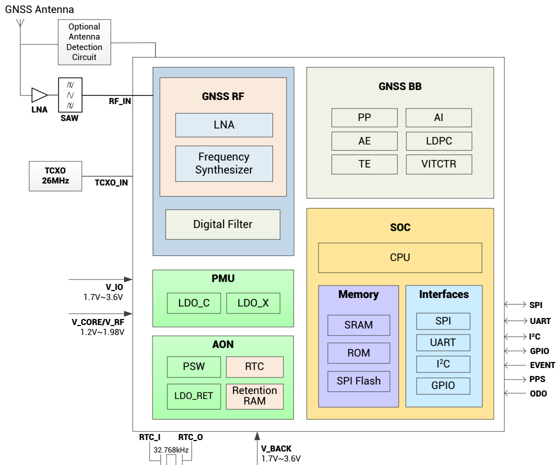
Figure 1-2 UC7510 Chip Block Diagram
