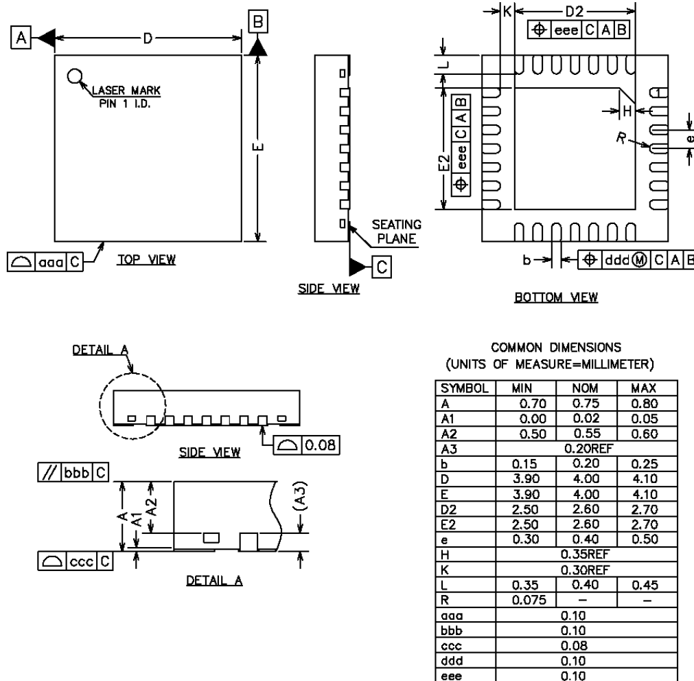
Figure 8-1 QFN28 Mechanical Specifications
